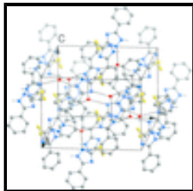
Fig. 2. Packing diagram of the title compound viewed down the a axis. O—H...N and N—H...O hydrogen bonds with the water molecule are shown with dashed lines.
